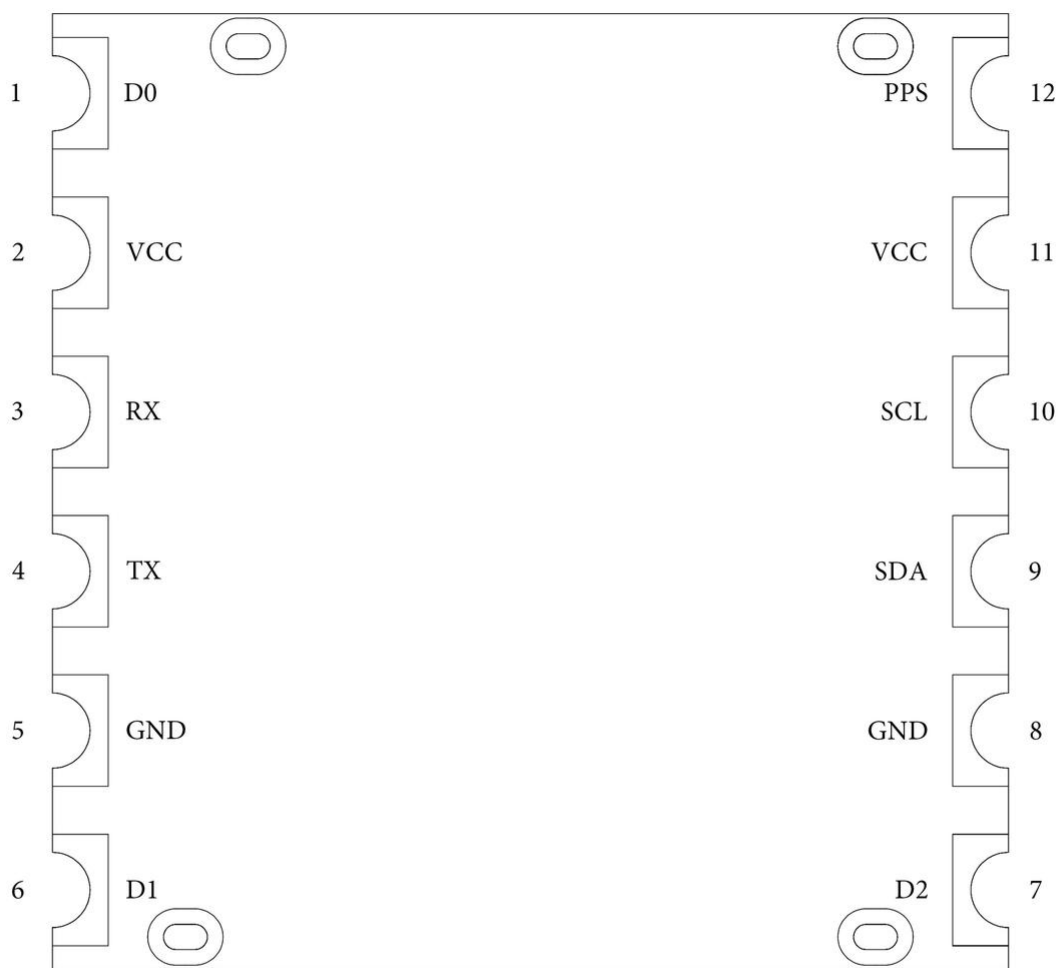
Z-FNIMU331 LAYOUT (TOP VIEW)
