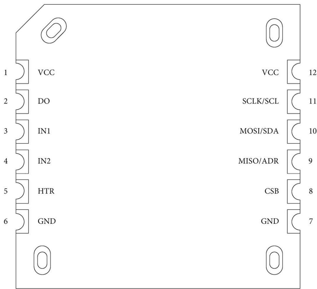
Z-FNIMU131 LAYOUT (TOP VIEW)
