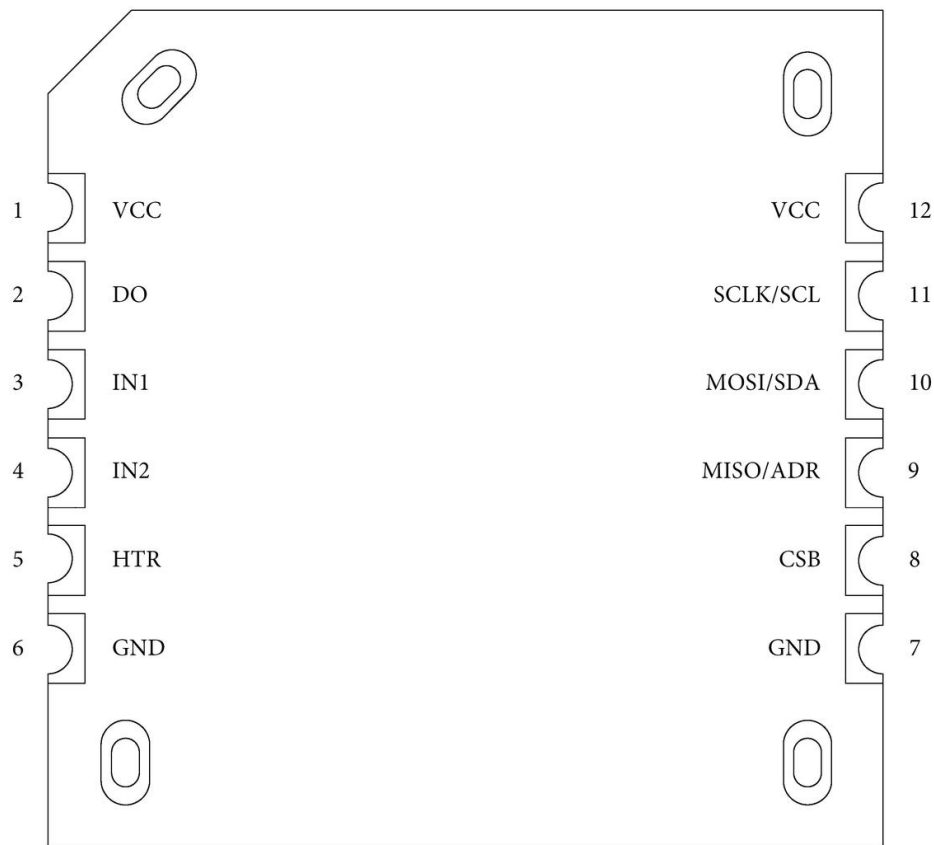
Z-FNIMU101 LAYOUT (TOP VIEW)
